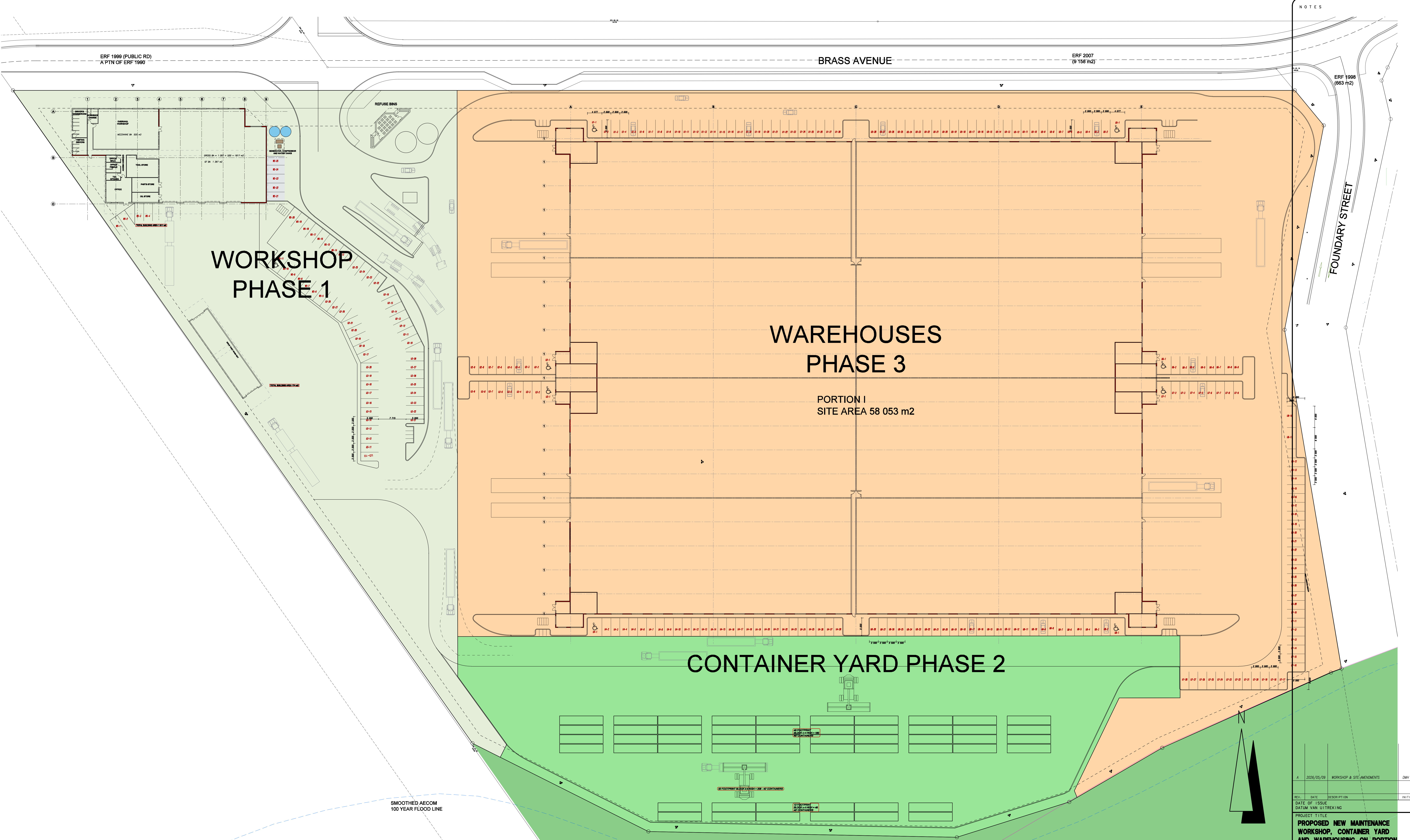
SITE DEVELOPMENT PLAN - PHASED LAYOUT SCALE 1:350
