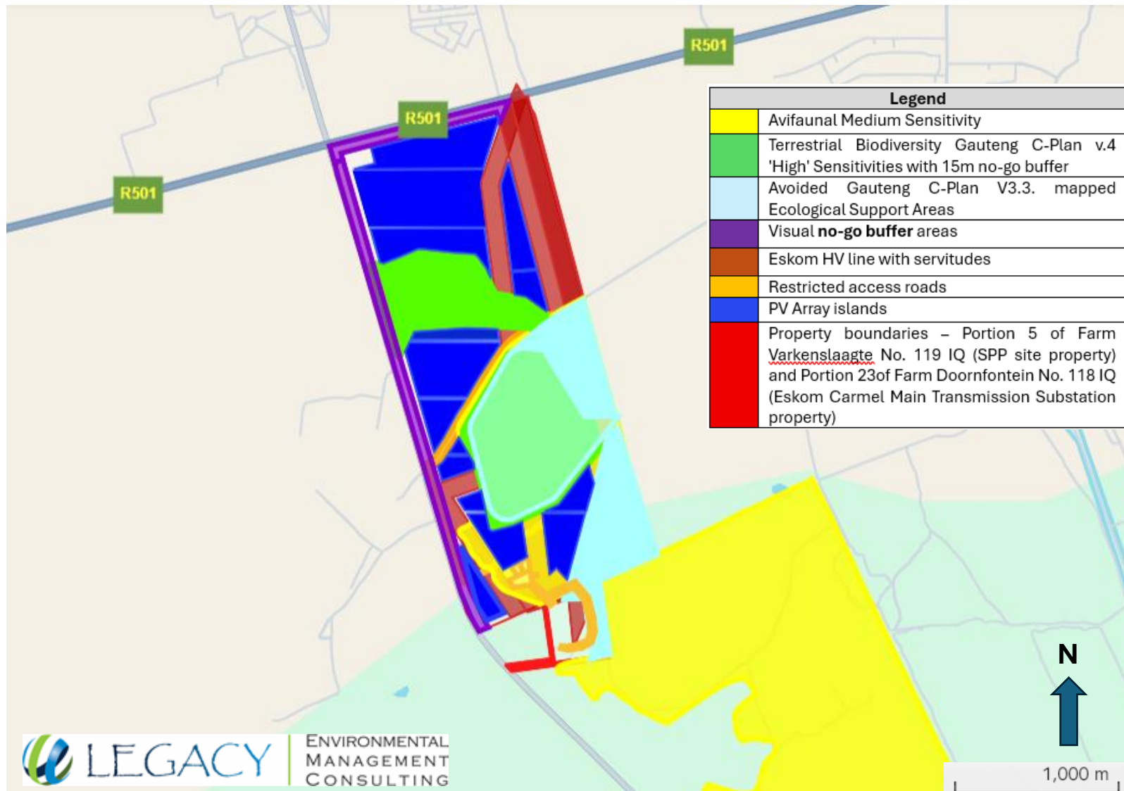
Figure 2: Carpe Diem North SPP final site layout map overlain with biodiversity sensitivities and other specialist sensitivities indicated for the site.
